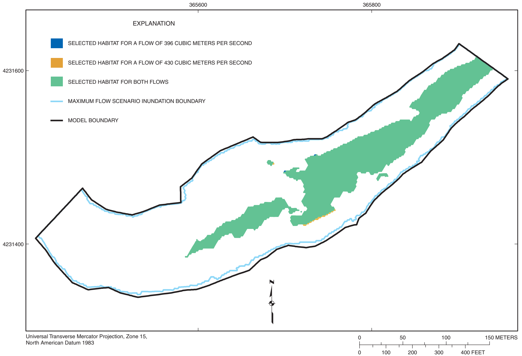
Figure 4-38. Selected habitat area distribution for habitat category 7 (paddlefish) at flows of 396 and 430 cubic meters per second at Marais des Cygnes River site MDC2.
